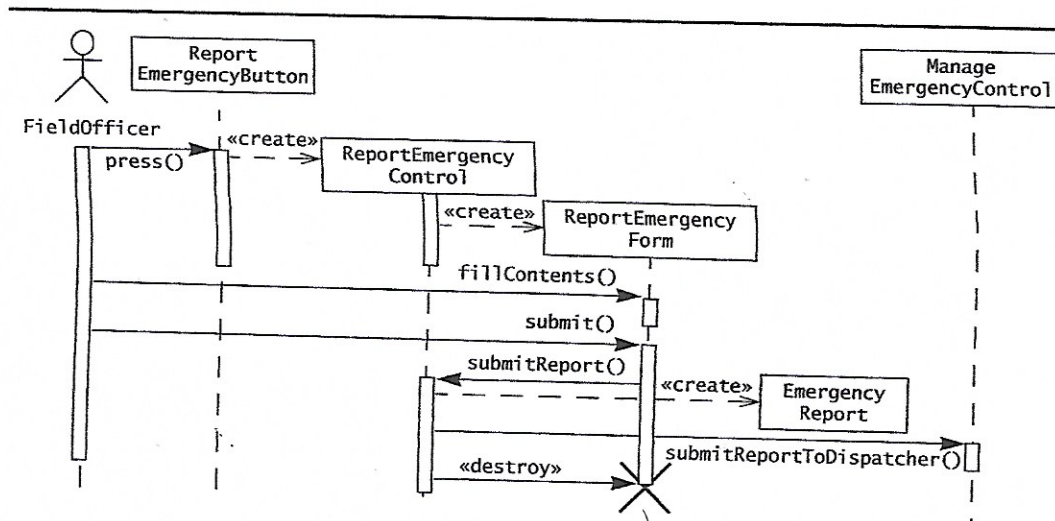
Figure 5-8 Sequence diagram for the ReportEmergency use case.
