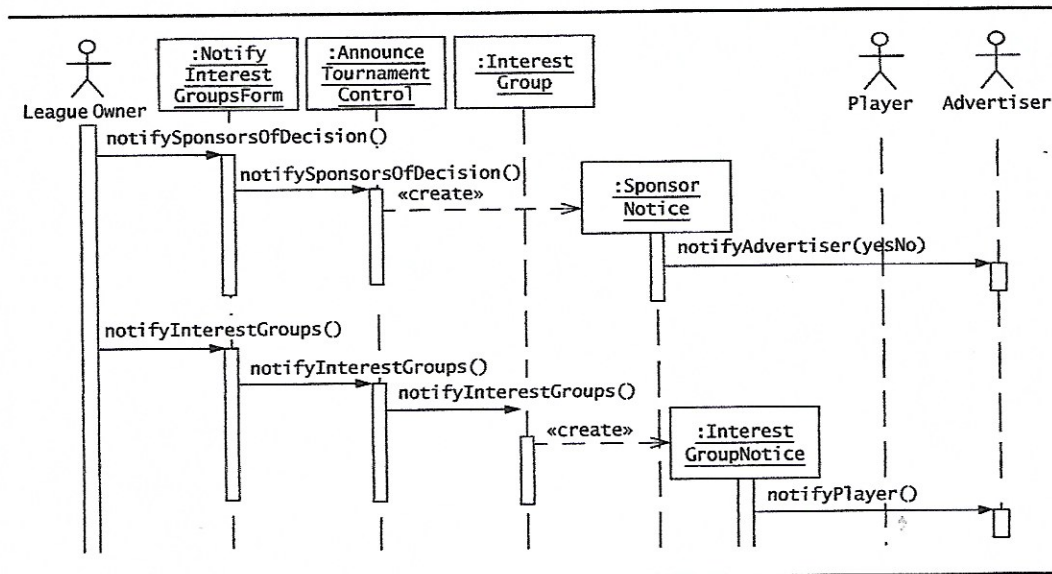
Figure 5-28 UML sequence diagram for AnnounceTournament use case, interest group workflow.
